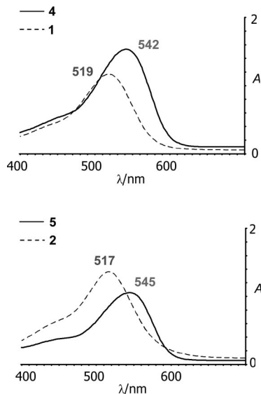
Figure 3. Visible spectra of oenin ( 1 ), malvidin ( 2 ) and the anthocyano-ellagitannins 4 and 5 in aqueous 1 M HCl solutions (pH 1). Estimated molar absorption coefficients ( \epsilon [L/mol·cm], 1 cm optical pathlength): 1 : \epsilon = 26000 , c = 4.8 \times 10^{-5} mol/L; 2 : \epsilon = 18400 , c = 6.7 \times 10^{-5} mol/L; 4 : \epsilon = 16300 , c = 9.4 \times 10^{-5} mol/L; 5 : \epsilon = 15700 , c = 7 \times 10^{-5} mol/L.
