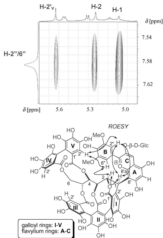
Figure 2. Diagnostic portion of the ROESY correlation map of 1-deoxyvescalagin-(1 \beta →8)-oenin ( 4 ) recorded in 1% TFA/MeOD (v/v). For an estimation of through-space interatomic distances, see Table 4.
