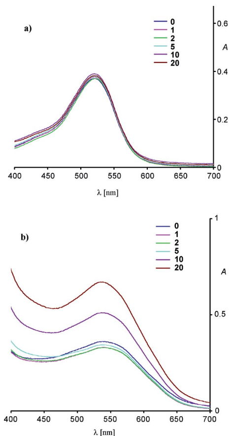
Figure 5. a) Visible spectra of oenin (1; 2.5 \times 10^{-5} M) and vescalagin (3) at 0, 1, 2, 5, 10, and 20 [copigment]/[pigment] molar ratios (pH = 1.0, T = 25 °C, optical pathlength = 1 cm, solvent = aqueous HCl/KCl buffer, ionic strength = 0.40 M). b) Visible spectra of oenin (1; 3.8 \times 10^{-4} M) and vescalagin (3) at 0, 1, 2, 5, 10, and 20 [copigment]/[pigment] molar ratios (pH = 3.2, T = 25 °C, optical pathlength = 1 cm; solvent = aqueous \text{KH}_2\text{PO}_4 buffer, ionic strength = 0.20 M).
