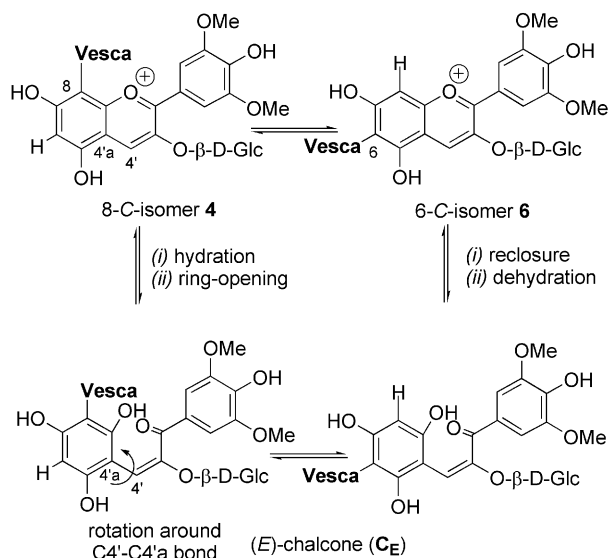
Scheme 4. Putative regioisomerization process of 1-deoxyvescalagin-(1 \beta →8)-oenin ( 4 ) to 1-deoxyvescalagin-(1 \beta →6)-oenin ( 6 ) in mildly acidic aqueous solutions [ Vesca = vescalagin ( 3 )-derived moiety].
