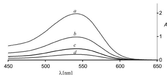
Figure 4. Visible spectra of 1-deoxyvescalagin-(1 \beta →8)-oenin ( 4 ) at different concentrations in aqueous 1 M HCl (pH 1). a) 1.2 \times 10^{-4} mol/L; b) 6.0 \times 10^{-5} mol/L; c) 3.1 \times 10^{-5} mol/L; d) 6.9 \times 10^{-6} mol/L (1 cm optical pathlength).
