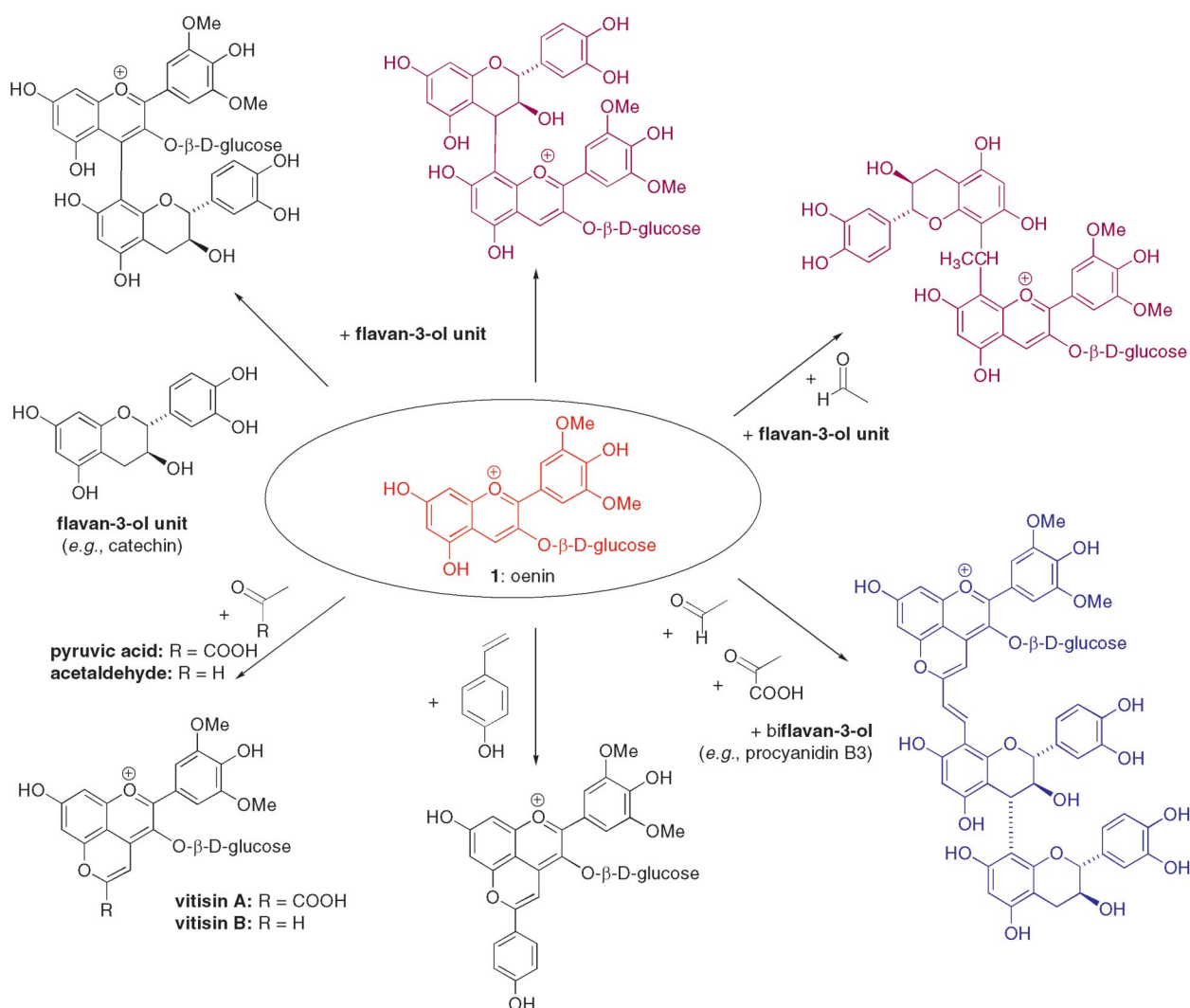
Scheme 1. From red grape oenin (1) to either bluer or more orangey wine genuine pigments. [2–7]
