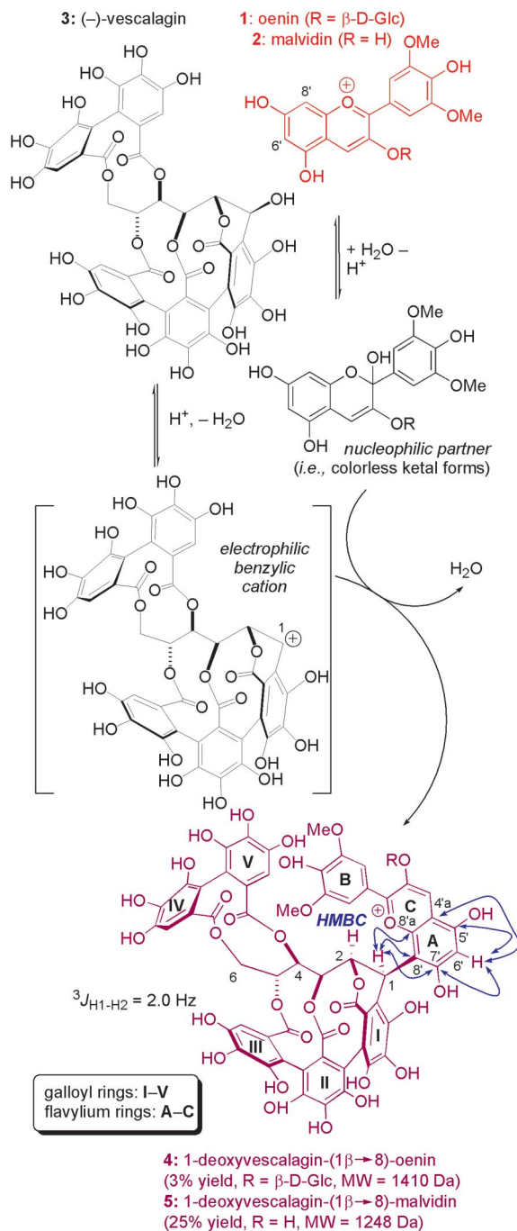
Scheme 2. Acid-catalyzed formation of the anthocyano-vescalagin condensation products 4 and 5 starting from vescalagin ( 3 ) and either oenin ( 1 ) or malvidin ( 2 ) in an acidic organic solution (i.e., 1.5% TFA/THF, v/v, 60 °C, 1–3 d).
