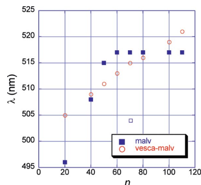
Figure 6. Evolution of the ZINDO-calculated first-allowed transition for malvidin ( 2 , malv) and 1-deoxyvescalagin-(1 \beta →8)-malvidin ( 5 , vesca-malv) as a function of the size of the active space ( n = m ).
