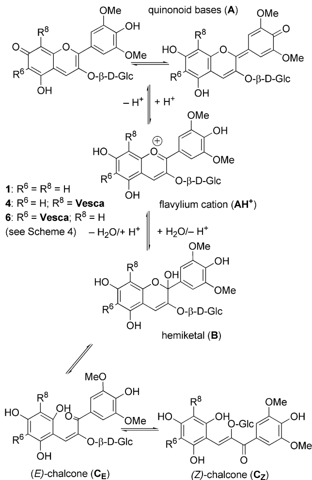
Scheme 3. Structural transformations of anthocyanins 1 and 4 in mildly acidic aqueous solutions [ Vesca = vescalagin ( 3 )-derived moiety].
