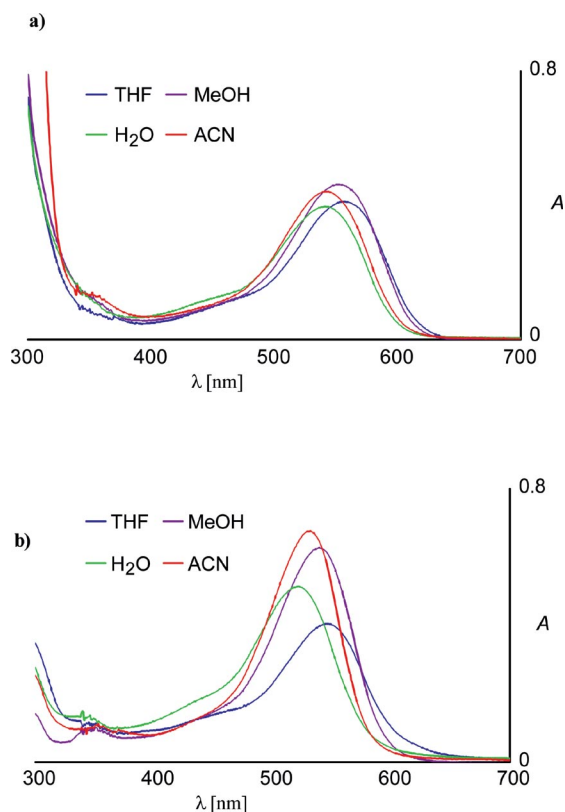
Figure 7. Evaluation of solvent effects on a) the visible spectra of 1-deoxyvescalagin-(1 \beta →8)-oenin ( 4 ; 2.4 \times 10^{-5} M) in four different solvents containing 1% TFA (v/v) ( T = 25 °C, optical pathlength = 1 cm) and b) the visible spectra of oenin ( 1 ; 2.0 \times 10^{-5} M) in four different solvents containing 1% TFA (v/v) ( T = 25 °C, optical pathlength = 1 cm).
