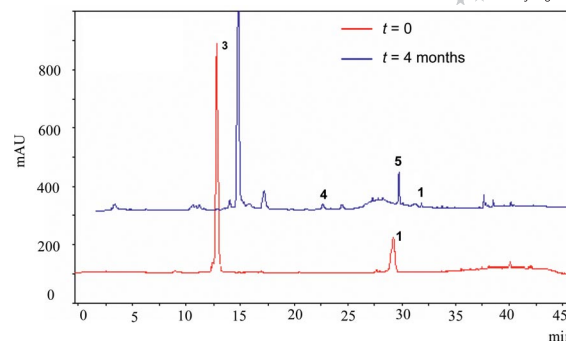
Figure 1. HPLC detection of the formation of adducts 4 and 5 starting from vescalagin ( 3 ) and oenin ( 1 ) in a wine model solution (i.e., 5 g/L of tartaric acid in 12% EtOH/H 2 O, v/v, adjusted to pH 3.2, room temp.). [12a]
